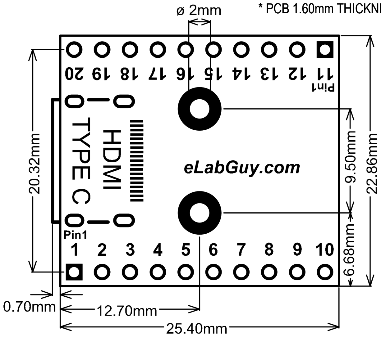
HDMI-CF-BO-V1A PCB outline Drawing
