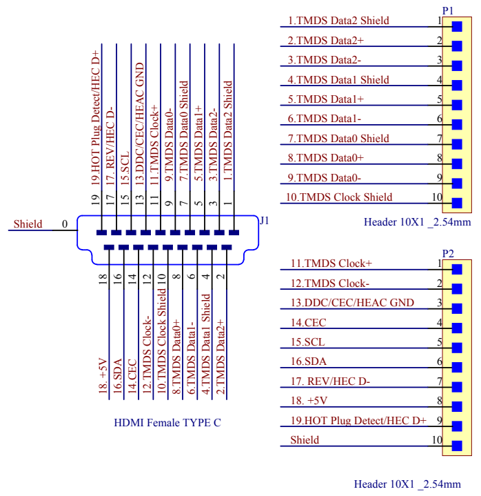
HDMI-CF-BO-V1A Schematic Diagram
